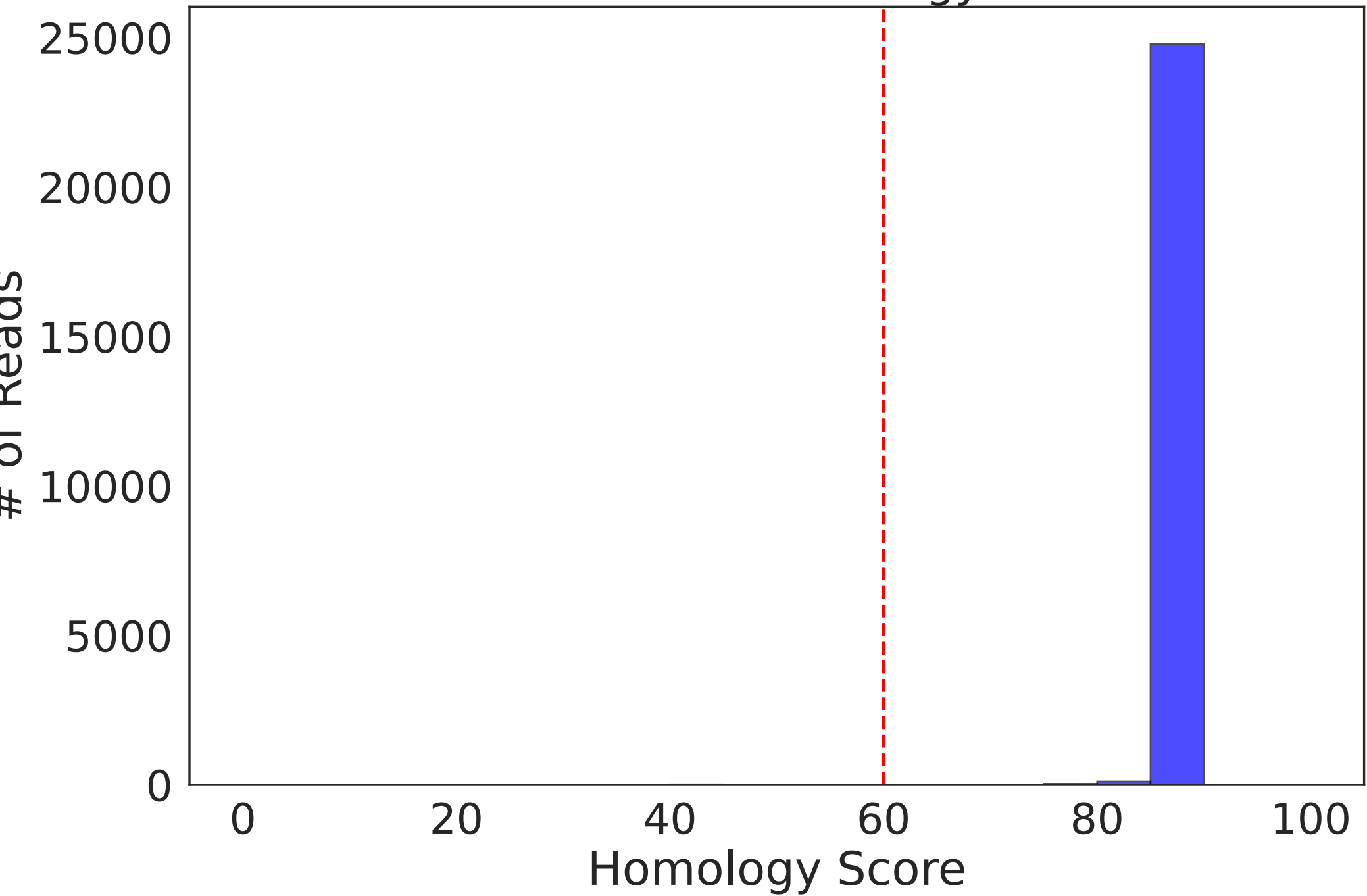
Distribution of Homology Scores
