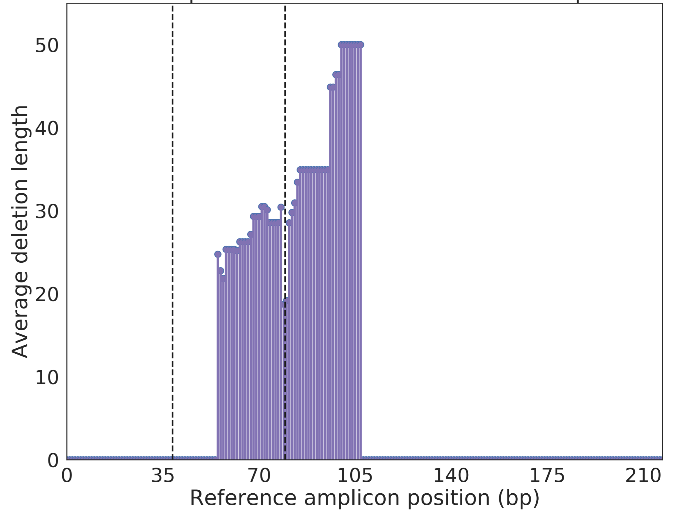
Position dependent deletion size: Scaffold-incorporated
