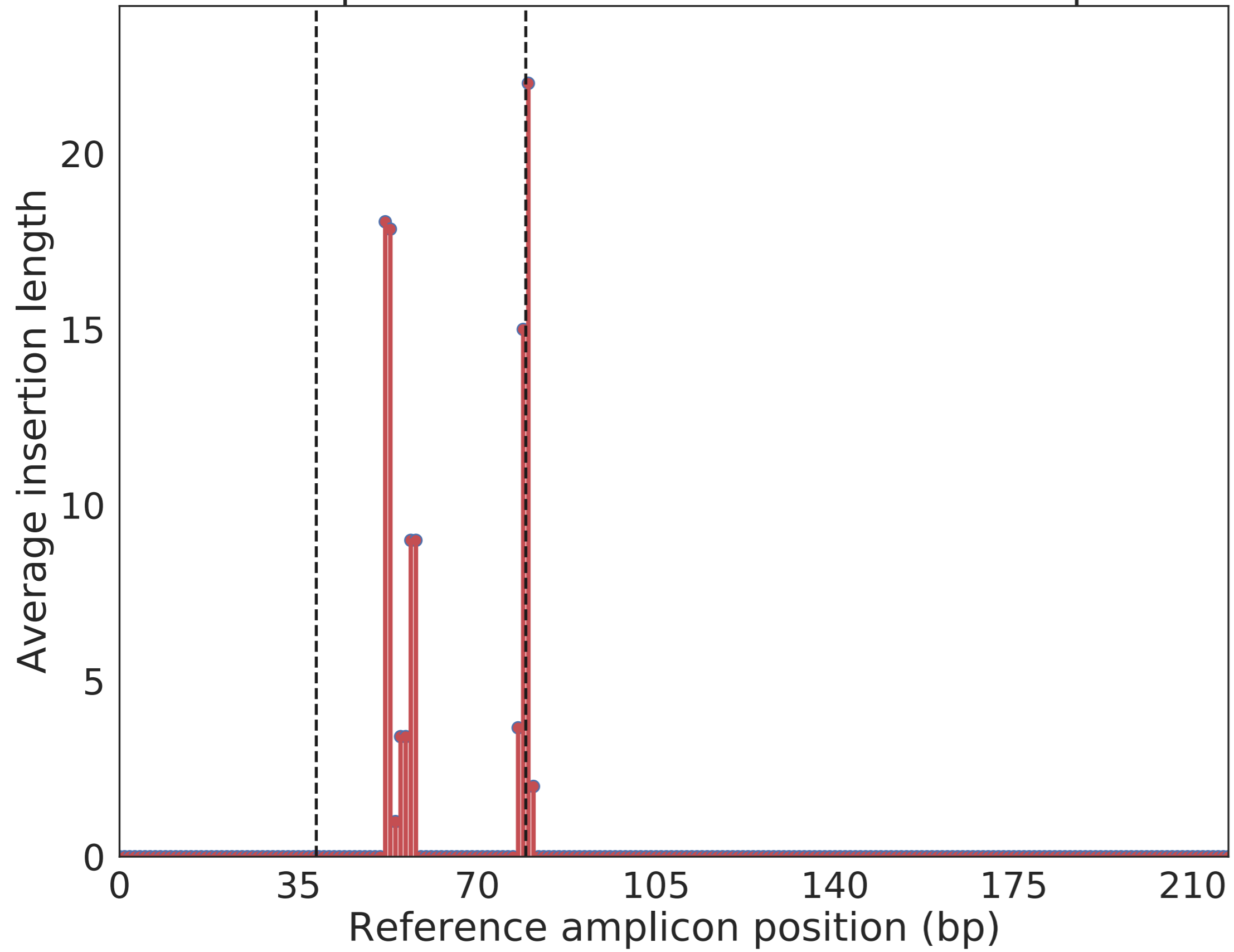
Position dependent insertion size: Scaffold-incorporated
