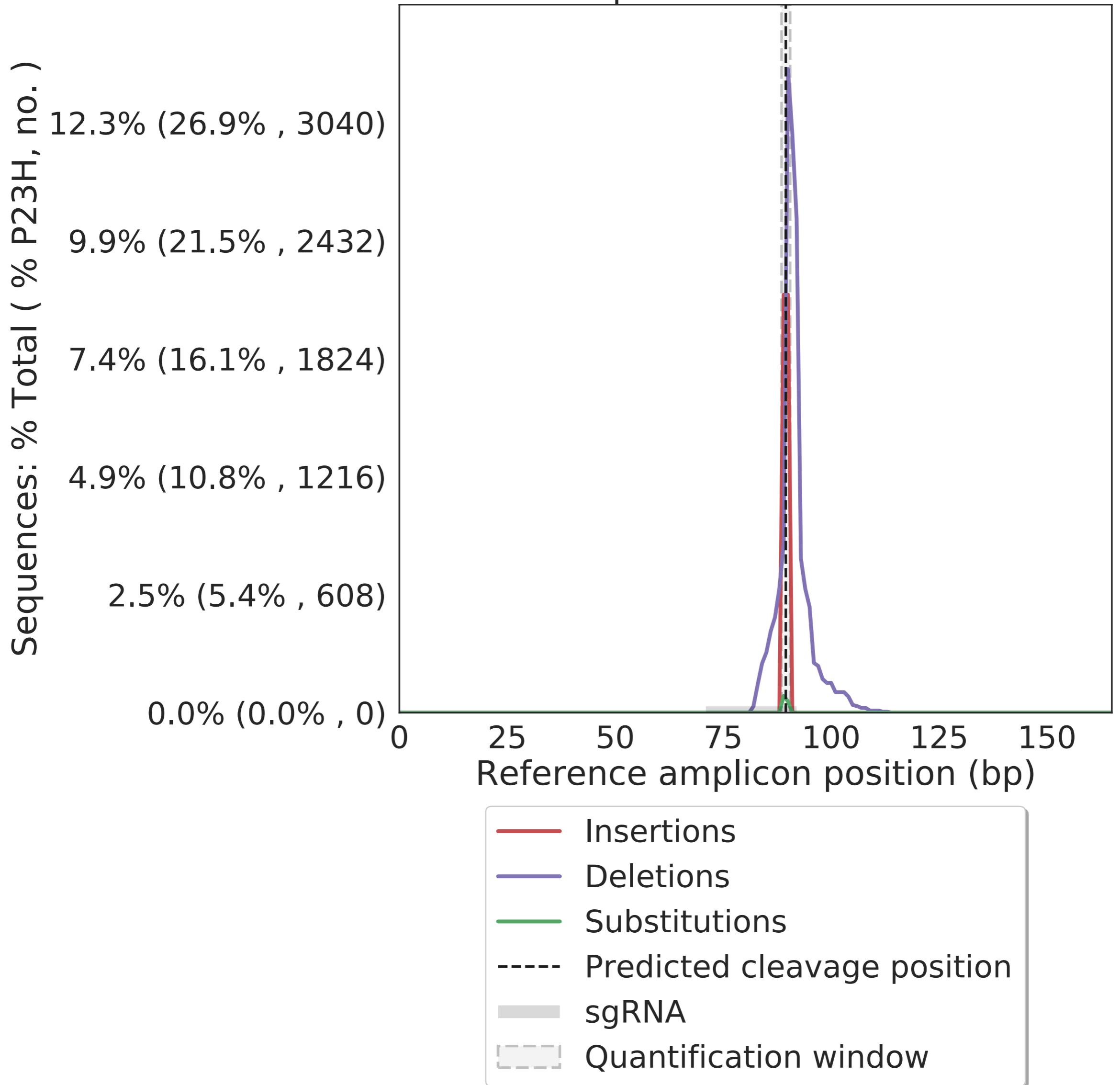
Mutation position distribution: P23H
