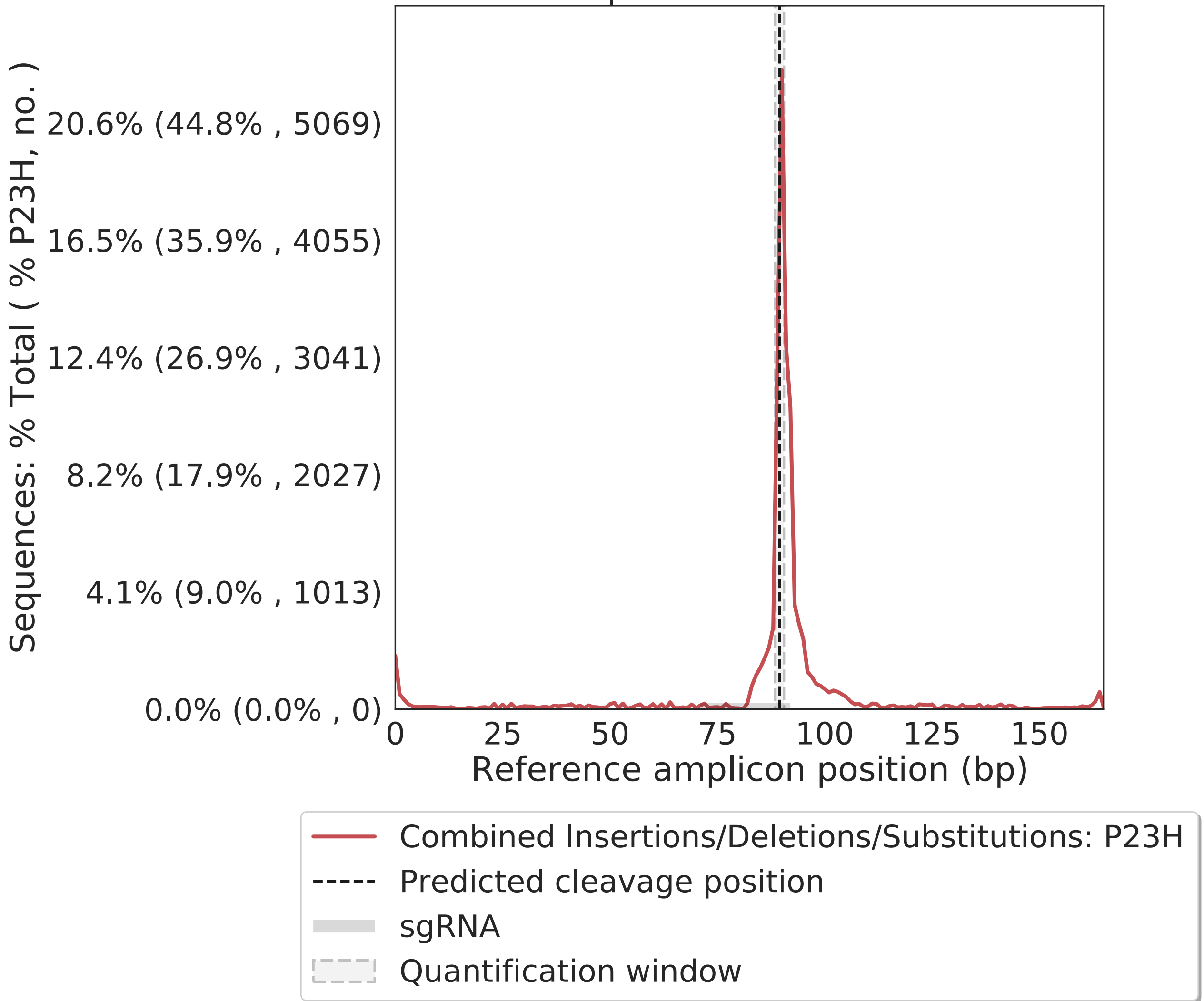
Mutation position distribution: P23H
