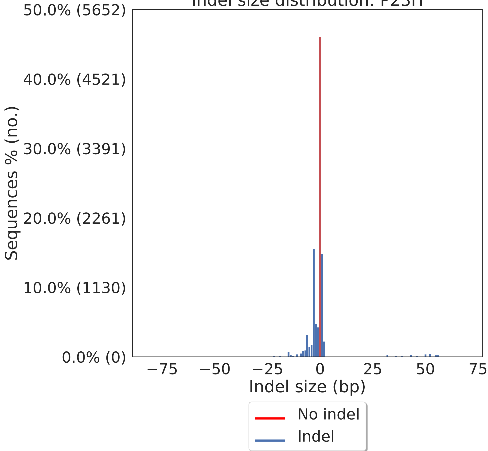
Indel size distribution: P23H
